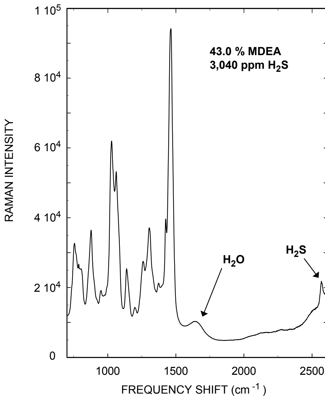
Raman spectrum of Methyldiethanolamine (MDEA). Sample contained 43.0 % MDEA and 3,040 ppm H 2 S.
